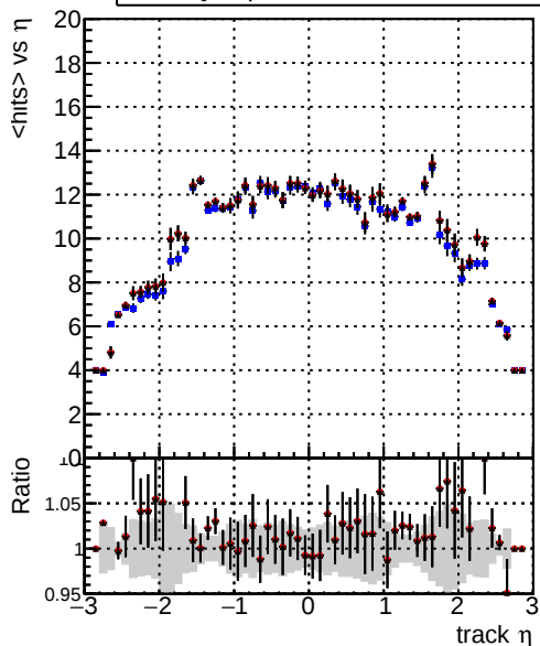
mean hits vs \eta Legend: DQMstep3_TT_CKF (blue line), DQMstep3_TT_default (red line), DQMstep3_TT_ckfPixelLess (black line)
