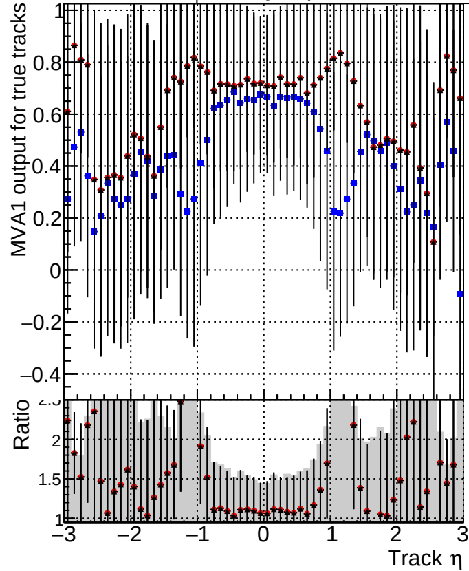
MVA1 of associated tracks (recoToSim) vs. track \eta Legend: DQMstep3_TT_CKF (blue squares) DQMstep3_TT_default (red stars) DQMstep3_TT_ckfPixelLess (black triangles)
