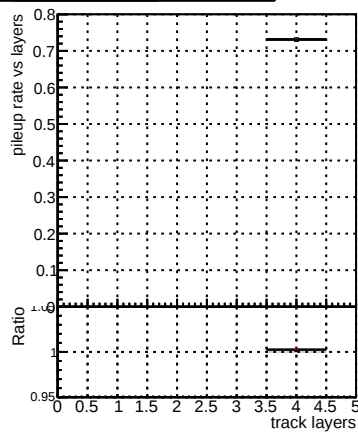
Pileup rate vs layers
