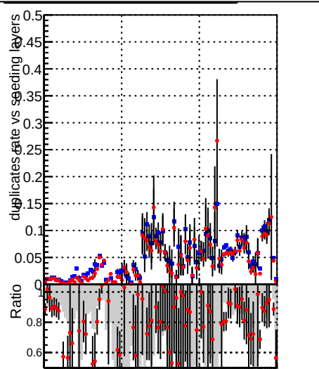
Duplicates rate vs seeding layers
