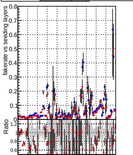
Fake rate vs. seeding layers
