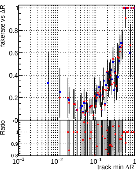
Fake rate vs \Delta R (track, jet) Legend: DQMstep3_TT_CKF (blue), DQMstep3_TT_CKF-tok (red)
