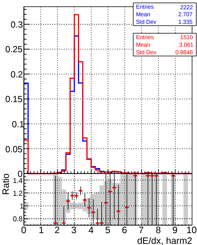
Legend: DQMstep3_TT_CKF (blue line with squares), DQMstep3_TT_CKF-tok (red line with circles)
