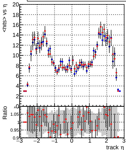
mean hits vs \eta Legend: DQMstep3_TT_CKF (blue line), DQMstep3_TT_CKF-tok (red line)
