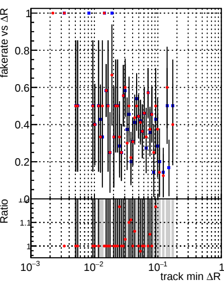
Fake rate vs \Delta R (track, jet) DQMstep3_TT_CKF DQMstep3_TT_CKF-tok
