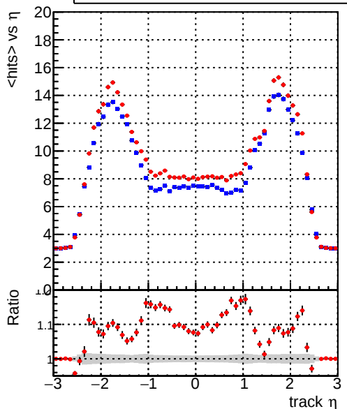
mean hits vs \eta Legend: DQMstep3_TT_CKF (blue line), DQMstep3_TT_CKF-tok (red line)
