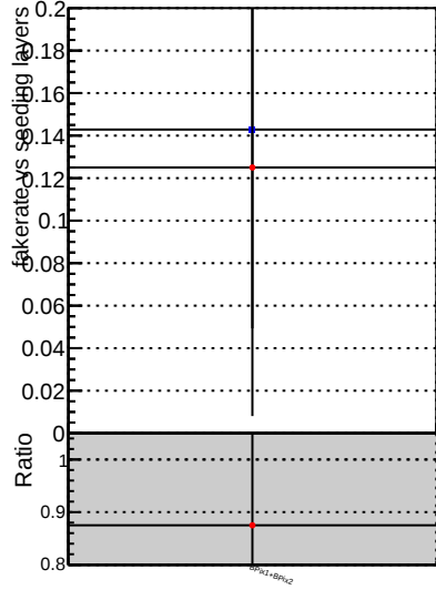
Fake rate vs. —●— DQMstep3_TT_CKF —●— DQMstep3_TT_CKF-tok
