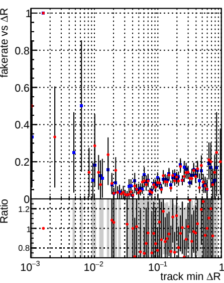
Fake rate vs \Delta R(\text{track, jet}) Legend: DQMstep3_TT_CKF (blue stars), DQMstep3_TT_CKF-tok (red stars)
