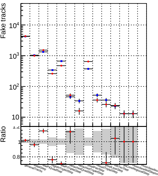
Number —●— DQMstep3_TT_CKF-tok
