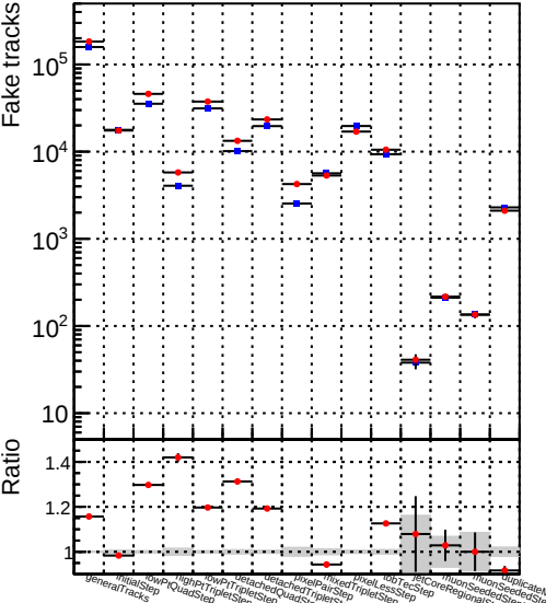
Number —●— DQMstep3_TT_CKF-tok
