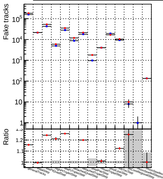
Number —●— DQMstep3_TT_CKF-tok
