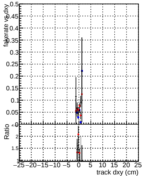
Legend for Fake rate vs dxy: DOMstep3 TT CKF (blue circles) DOMstep3 TT default (red circles) DOMstep3 TT NEWT (black circles) DOMstep3 TT default NEWT (grey circles)
