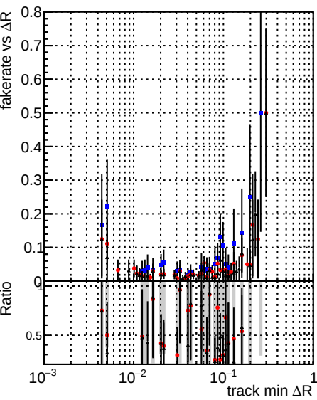
Fake rate vs \Delta R(\text{track, jet}) Legend: DOMstep3_TT_CKF (blue circles) DOMstep3_TT_default (red circles) DOMstep3_TT_defaultNEWT (black circles)
