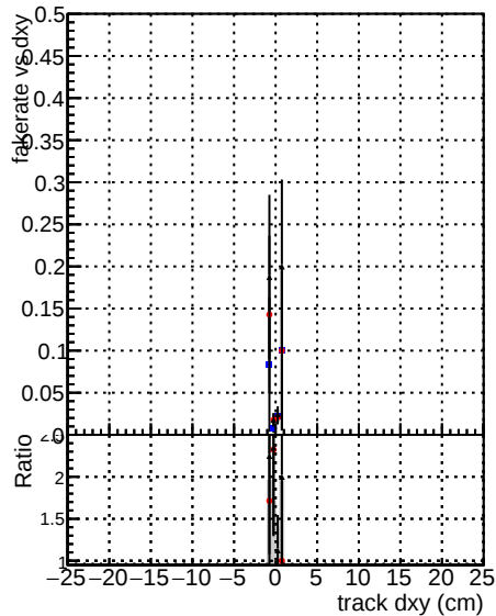
DOMstep3 TT CKF Fake rate vs d —●— —●— Duplicates Rate vs Dxy —●— —●— Pileup rate vs dxy —●— —●—
