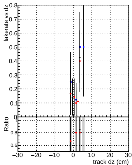
Legend for Fake rate vs d, Duplicates Rate vs Dxy, and Pileup rate vs dxy plots: DOMstep3 TT CKF (Blue line with dots) DOMstep3 TT default (Red line with dots) DOMstep3 TT defaultNEWT (Black line with dots)
