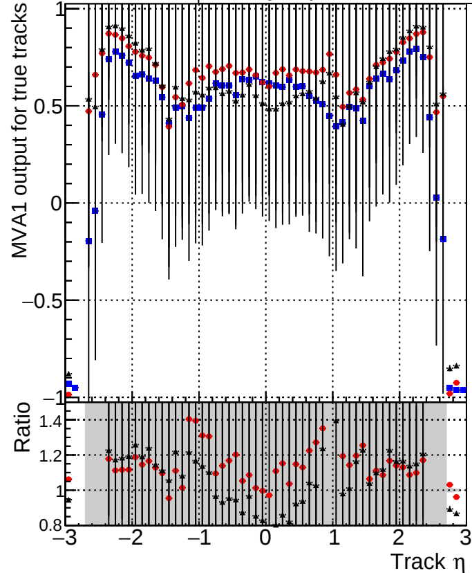
MVA1 of associated tracks (recoToSim) vs. track \eta Legend: DQMstep3_TT_CKF (blue squares) DQMstep3_TT_default (red diamonds) DQMstep3_TT_defaultNEWT (black stars)
