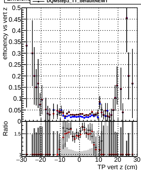
Efficiency vs. TP vert z (cm)
