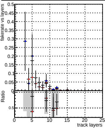
Fake rate vs hit Legend: DQMstep3_TT_CKF (blue dots) DQMstep3_TT_default (red dots) DQMstep3_TT_defaultNEWT2 (black dots)
