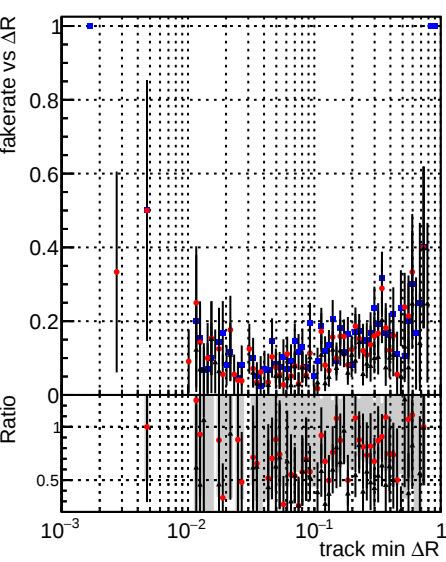
Legend: DQMstep3_TT_CKF (blue dots), DQMstep3_TT_default (red dots), DQMstep3_TT_defaultNEW2 (black dots with error bars)
