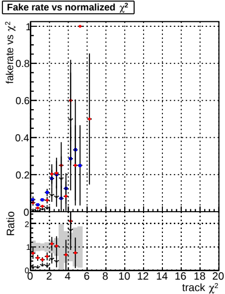
Fake rate vs. ● DOMstep3 ● TT CKF ● default + DOMstep3 + TT CKF + default
