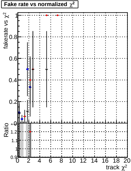
Fake rate vs. \chi^2 Legend: DOMstep3 (blue), CKF (red), default (black)
