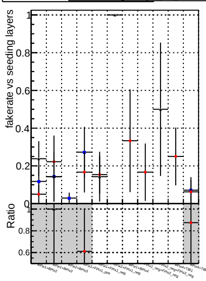
Fake rate vs. DOMstep3 CKF default
