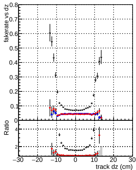
Fake rate vs dz DOMstep3 TT CKF DOMstep3 default NEWT3
