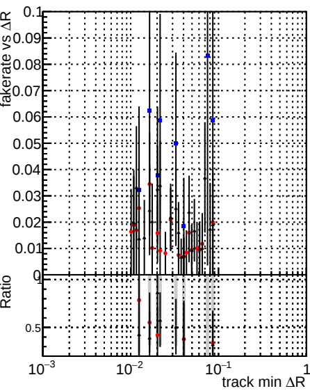
Fake rate vs \Delta R(\text{track}, \text{jet}) Legend: DOMstep3_TT_CKF (blue dots) DOMstep3_TT_default (red dots) DOMstep3_TT_defaultNEWT3 (black dots)
