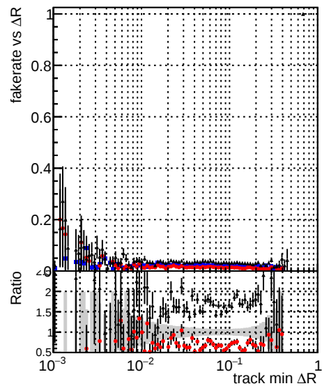
Legend: DQMstep3_TT_CKF (black line with dots) DQMstep3_TT_default (red line with dots) DQMstep3_TT_defaultNEWT3 (blue line with dots)
