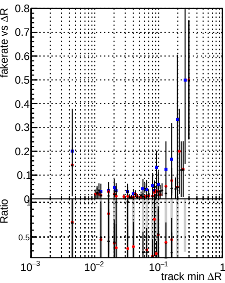
Fake rate vs \Delta R(\text{track, jet}) Legend: - DOMstep3 TT CKF (blue dots) - DOMstep3 TT default (red dots) - DOMstep3 TT defaultNEW3 (black dots)
