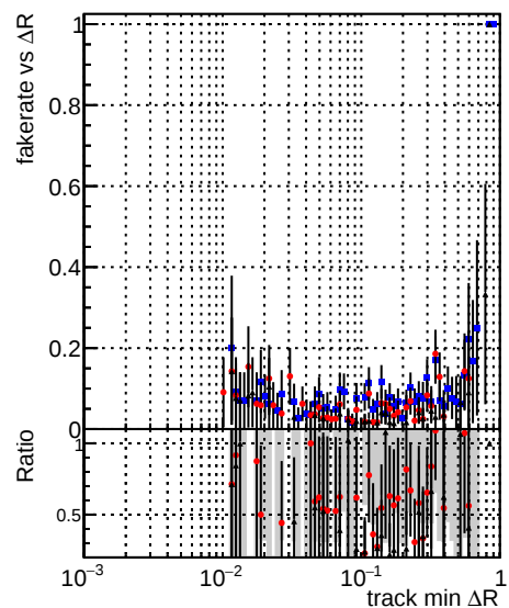
Legend: DOMstep3_TT_CKF (blue circles) DOMstep3_TT_default (red circles) DOMstep3_TT_defaultNEWT3 (black circles)
