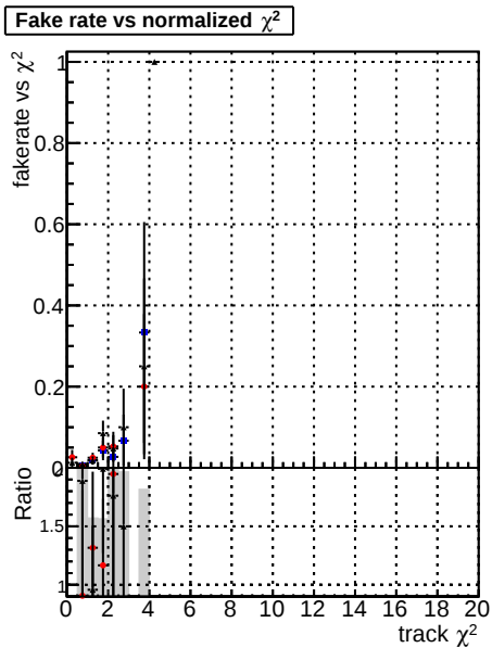
Fake rate vs. \chi^2 for DOMstep3, CKF, default, and NEWT3
