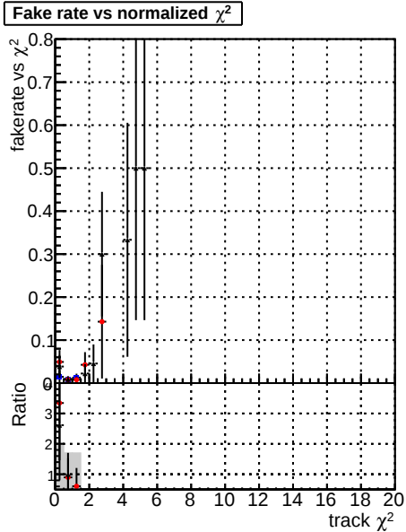
Fake rate vs. DOMstep3 CKF default Duplicate Rate vs. DOMstep3 CKF default Pileup rate vs. DOMstep3 CKF default
