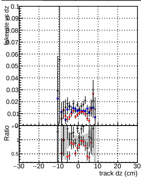
Fake rate vs dz DOMstep3 TT CKF default defaultNEWT3
