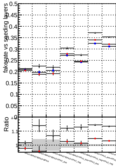
Fake rate vs. DOMstep3 CKF default default default NEWT203
