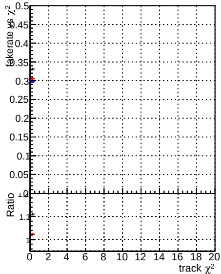
Fake rate vs. DOMstep3 CKF default default default NEWT203
