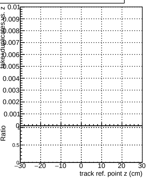
fake+duplicates vs track ref. point z
