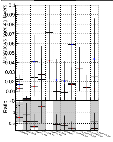
Fake rate vs. DOMstep3 CKF default NEWT203
