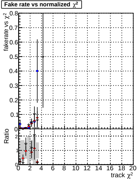
Fake rate vs. DOMstep3 CKF default NEWT203
