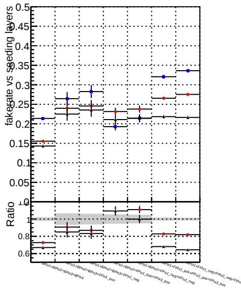
Fake rate vs. DOMstep3 CKF DOMstep3 default NEWT203
