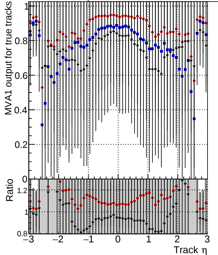
MVA1 of associated tracks (recoToSim) vs. track \eta Legend: DQMstep3_TT_CKF (blue squares) DQMstep3_TT_default (red circles) DQMstep3_TT_defaultNEWT203 (black stars)
