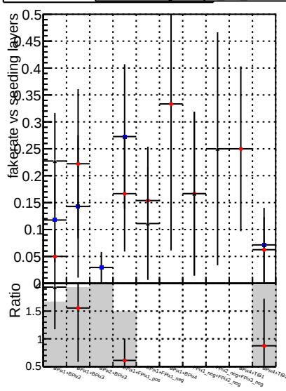
Fake rate vs. Legend: DOMstep3 (blue dots), TT CKF (black crosses), default (red dots) Legend: DOMstep3 (blue dots), TT CKF (black crosses), default (red dots) Legend: DOMstep3 (blue dots), TT CKF (black crosses), default (red dots)
