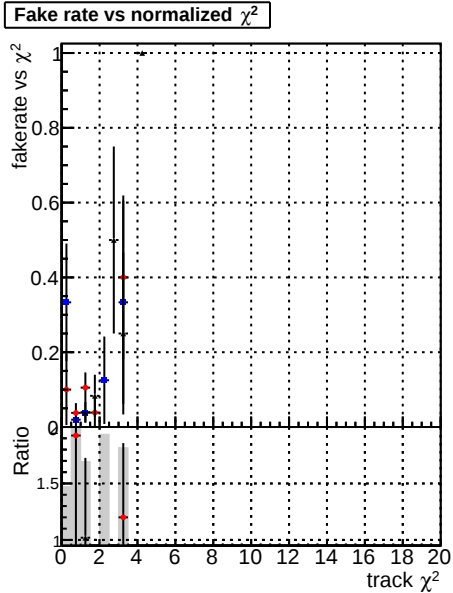
Fake rate vs. Legend: DOMstep3 (blue dots), TT CKF (black crosses), default (red dots) Legend: DOMstep3 (blue dots), TT CKF (black crosses), default (red dots) Legend: DOMstep3 (blue dots), TT CKF (black crosses), default (red dots)
