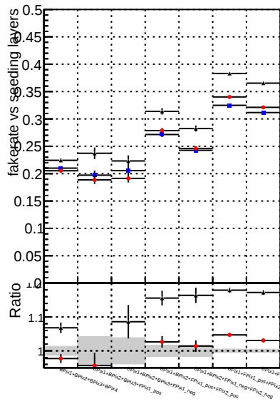
Fake rate vs. DOMstep3 TT CKF default default DOMstep3 defaultNEW20
