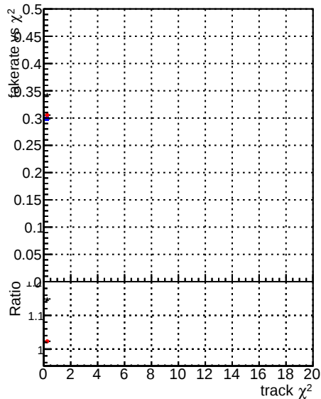
Fake rate vs. DOMstep3 TT CKF default default DOMstep3 defaultNEW20
