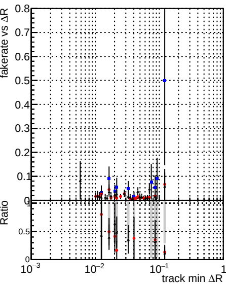
Fake rate vs \Delta R(\text{track, jet}) Legend: - DOMstep3_TT_CKF (blue) - DOMstep3_TT_default (red) - DOMstep3_TT_defaultNEW20 (black)
