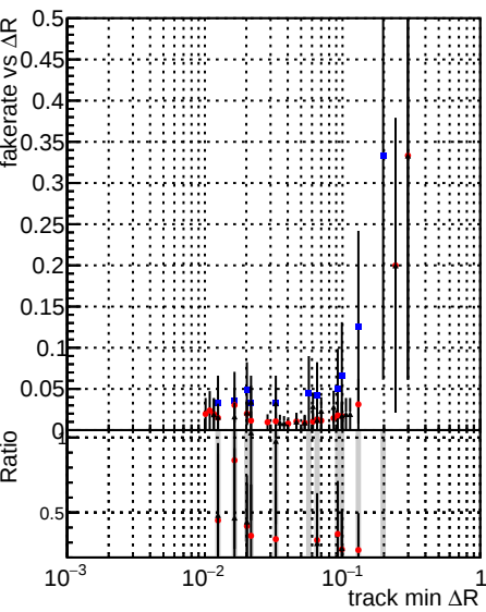
Fake rate vs \Delta R(\text{track, jet}) Legend: DQMstep3 TT CKF (blue dots) DQMstep3 TT default (red dots) DQMstep3 TT defaultNEW20 (black dots)
