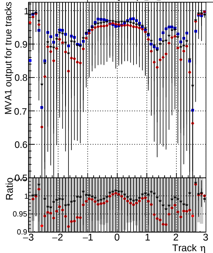
MVA1 of associated tracks (recoToSim) vs. track \eta Legend: ■ DQMstep3_TT_CKF ● DQMstep3_TT_default ▲ DQMstep3_TT_defaultNEWT20
