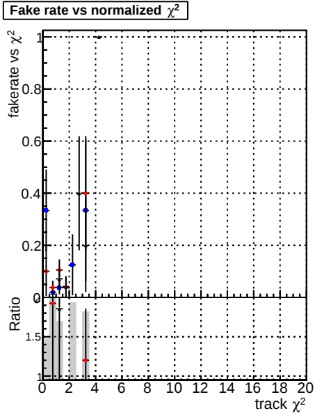
Fake rate vs. \chi^2 for different track reconstruction methods: DOMstep3, CKF, default, and NEWT20.
