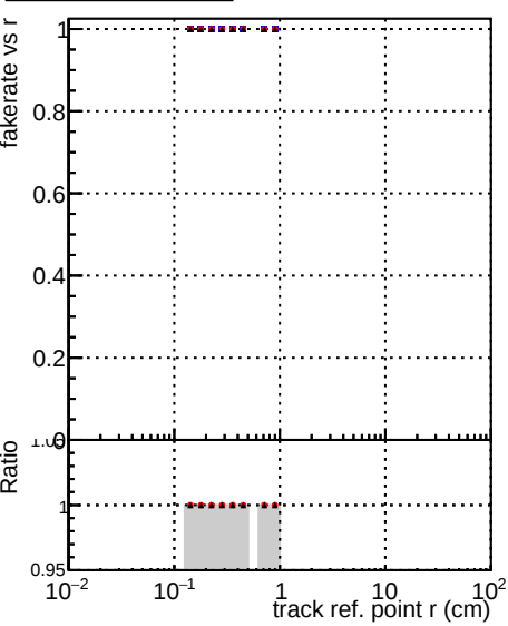
Fake rate vs v Legend: DOMstep3_TT_CKF (blue line with dots) DOMstep3_TT_default (red line with dots) DOMstep3_TT_defaultNEWTreweight (black line with dots)
