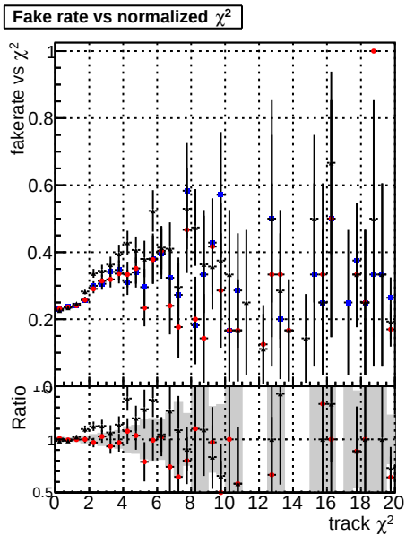
Fake rate vs. \chi^2 for tt CKF, DOMstep3, and default. The ratio is shown in the bottom panel.
