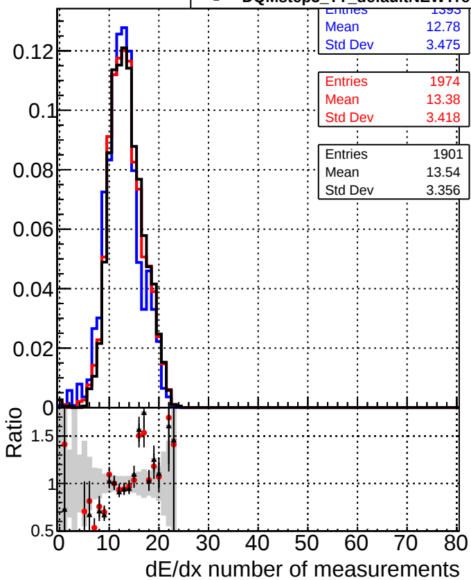
Legend for bottom row plots: DQMstep3_TT_CKF (blue line with squares) DQMstep3_TT_default (red line with circles) DQMstep3_TT_defaultNEWTreweight (black line with crosses)
