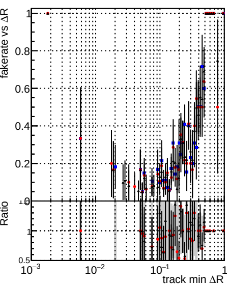
Fake rate vs ΔR(track, jet) Legend: DQMstep3 TT CKF (blue dots) DQMstep3 TT default (red dots) DQMstep3 TT defaultNEWTweight (black line with error bars)
