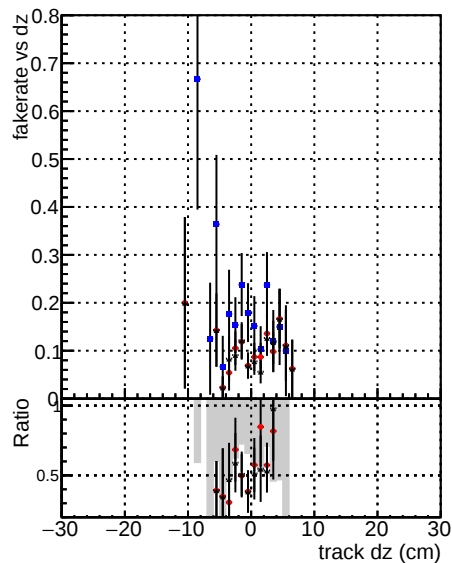
Fake rate vs dz —•— DOMstep3 TT CKF —•— DOMstep3 TT default —•— DOMstep3 TT defaultNEWTreweight
