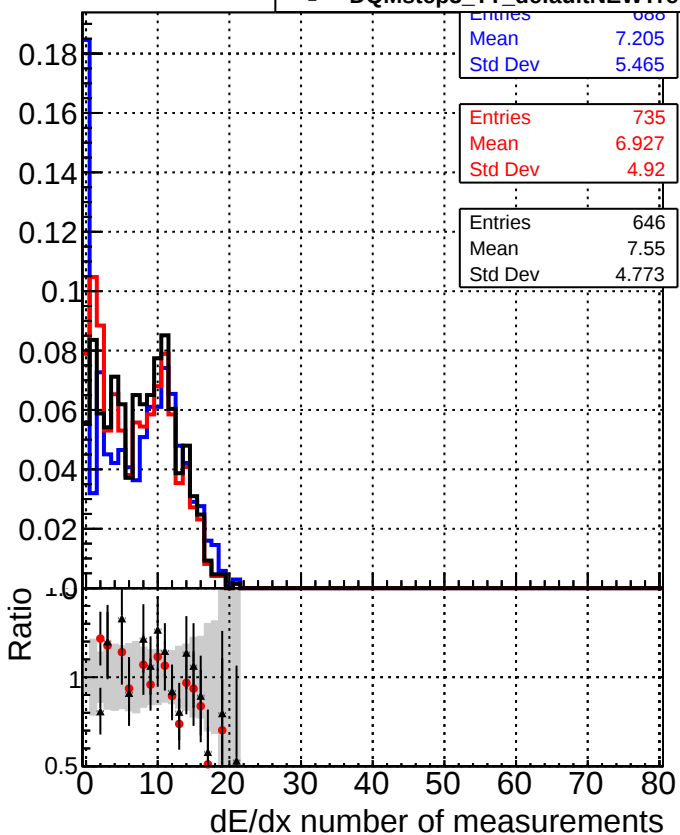
Legend for dE/dx number of measurements: DQMstep3_TT_CKF (Blue line with squares) DQMstep3_TT_default (Red line with circles) DQMstep3_TT_defaultNEWTreweight (Black line with crosses)
